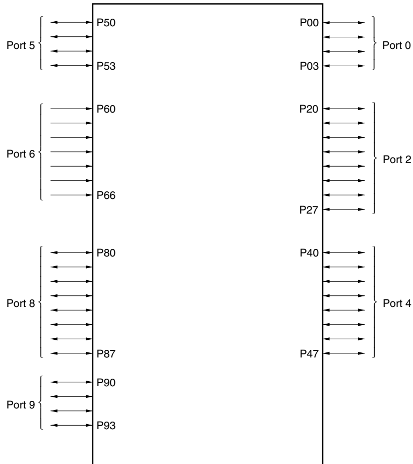
Figure 4-1. Port Types
