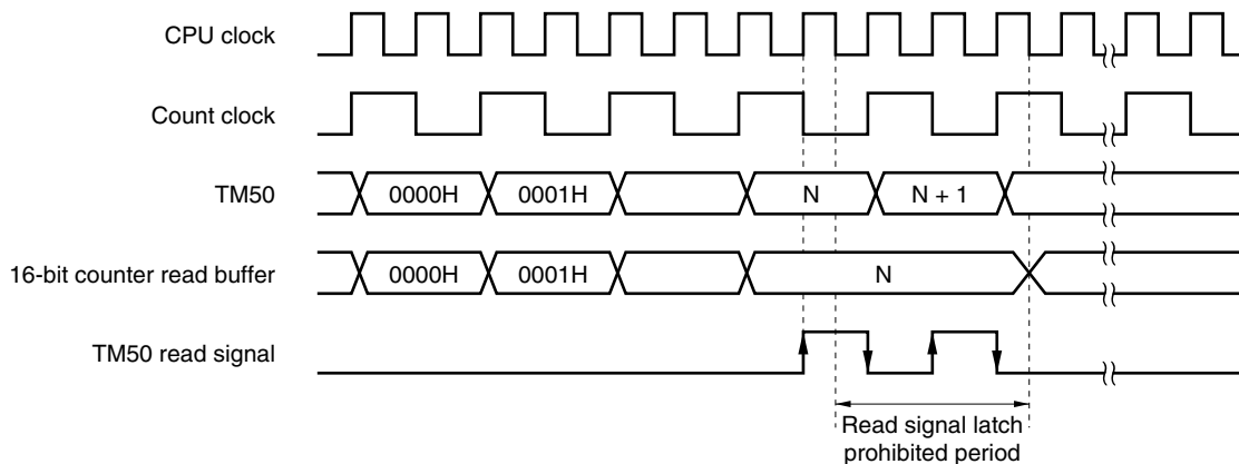
Figure 6-10. Readout Timing of 16-Bit Timer Counter 50
