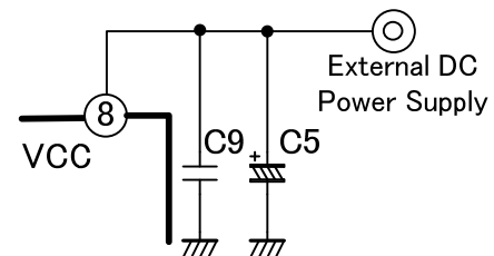
Fig.29 VCC pin circuit (2)
