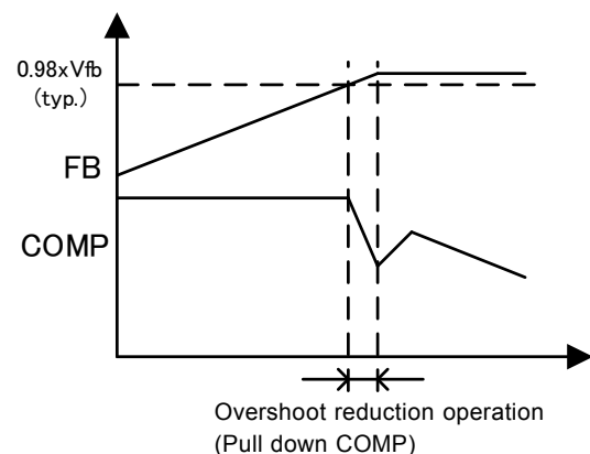
Fig.6 Overshoot reduction operation
