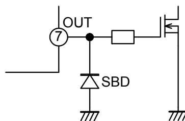
Fig.30 Protection circuit of OUT pin against the negative voltage
