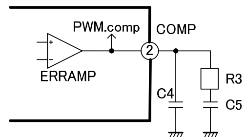
Fig.17 COMP pin circuit
