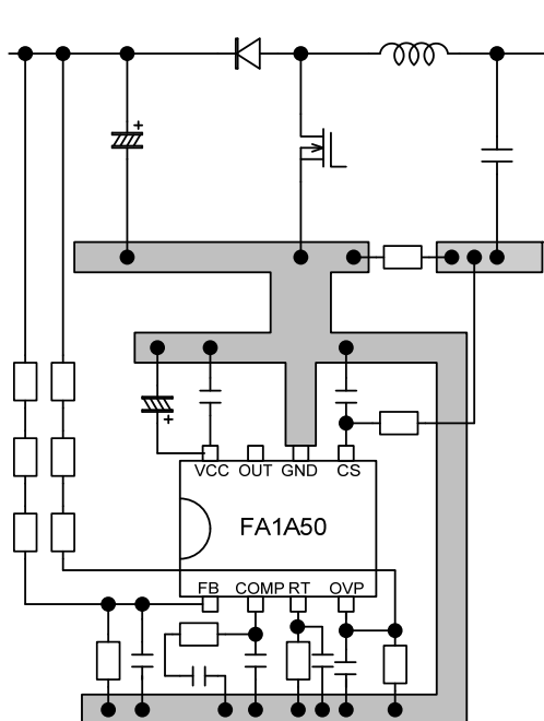
Fig.36 Good example of GND wiring around IC
