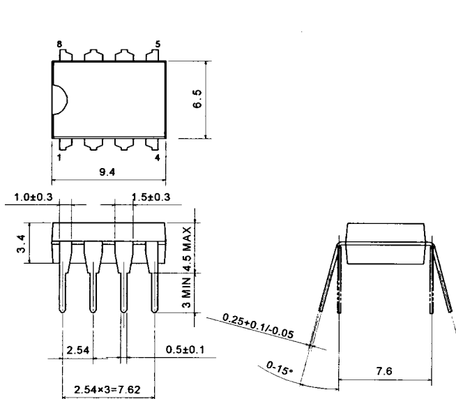
DIP-8 (FA5516P/FA5517P/FA5518P)
