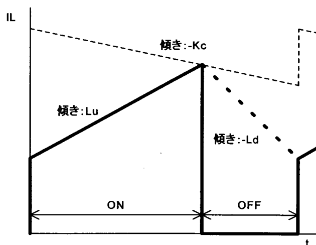
Fig.42 Inductor current without slope compensation
