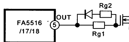
Fig.39 Gate circuit (2)
