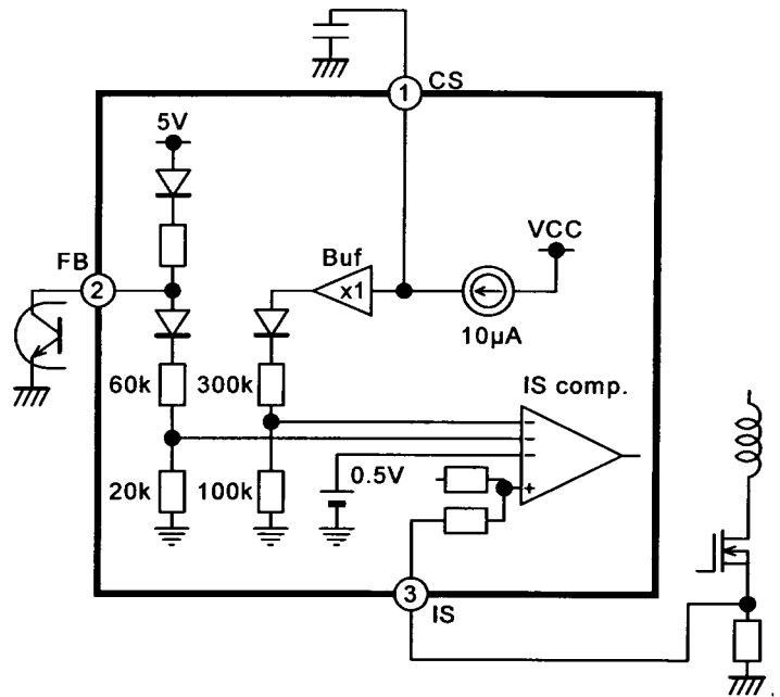
Fig.7 Current comparator
