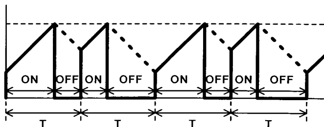
Fig.40 Inductor current without slope compensation
