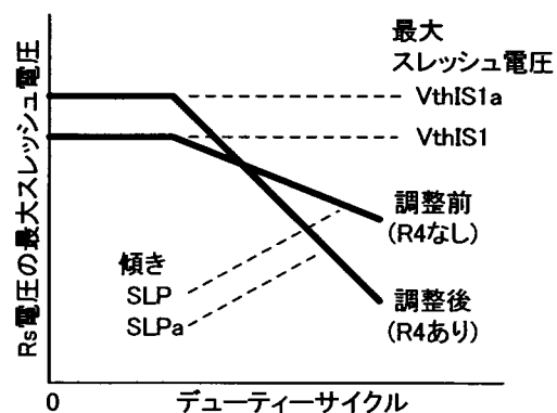
Fig.33 Maximum threshold voltage after adjustment
