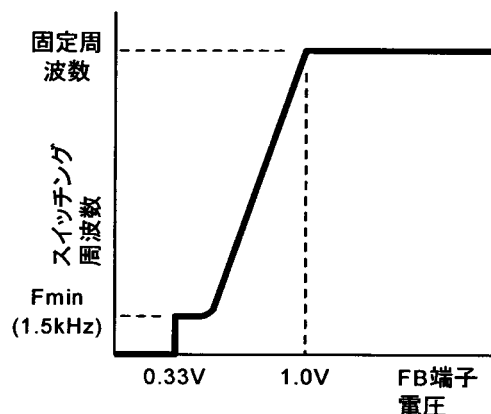
Fig.4 Oscillating frequency
