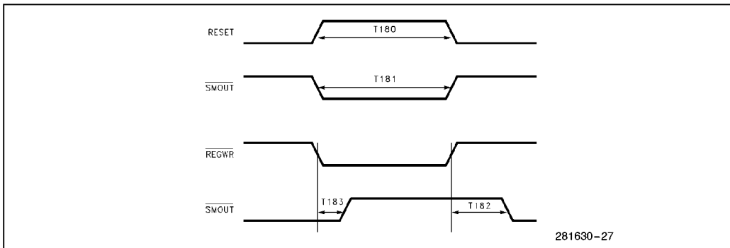
Figure 11-17. \overline{\text{SMOUT}} Timing
