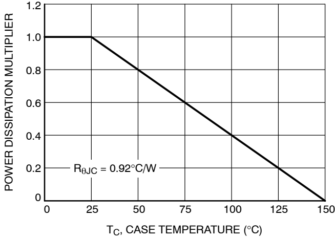
Figure 5. Normalized Power Dissipation vs. Case
