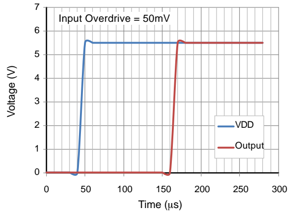
Figure 13. Power-Up Delay
