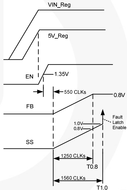
Figure 30. Typical Soft-Start Timing Diagram
