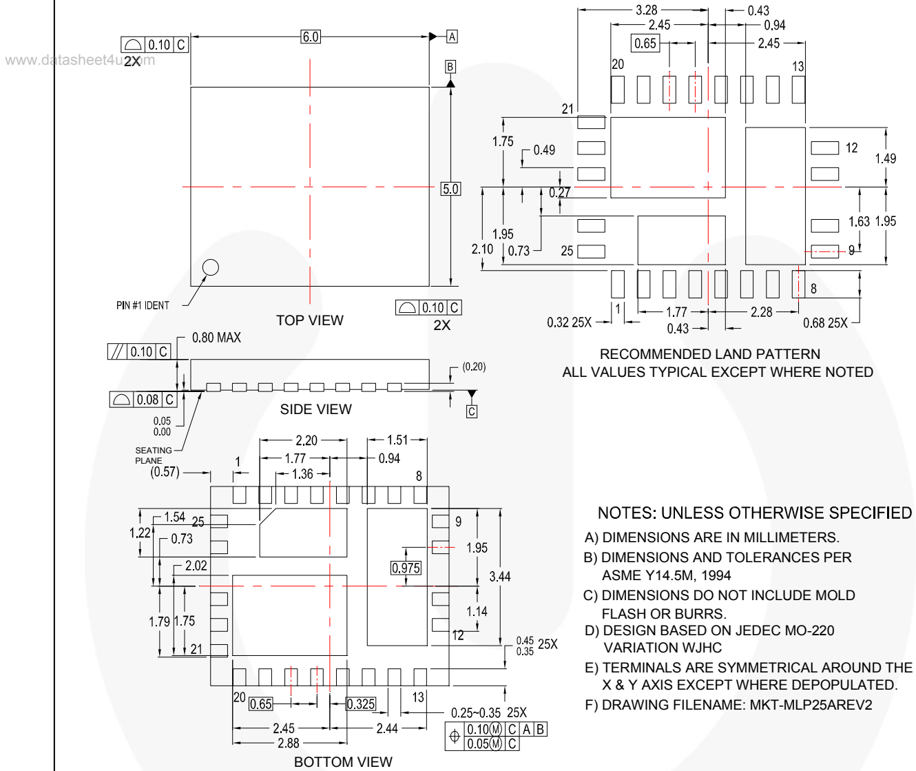
Figure 38. 5x6mm Molded Leadless Package (MLP)
