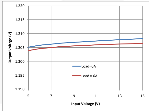
Figure 14. Line Regulation
