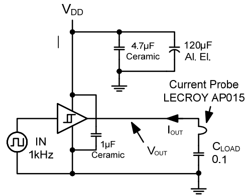
Figure 20. Quasi-Static I_{\text{OUT}} / V_{\text{OUT}} Test Circuit
