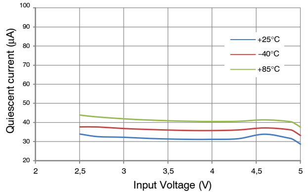
Figure 8. Quiescent Current
