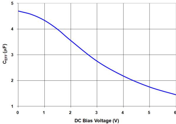
Figure 49. C EFF for 4.7 μF, 0603, X5R, 6.3 V (Murata GRM188R60J475K)
