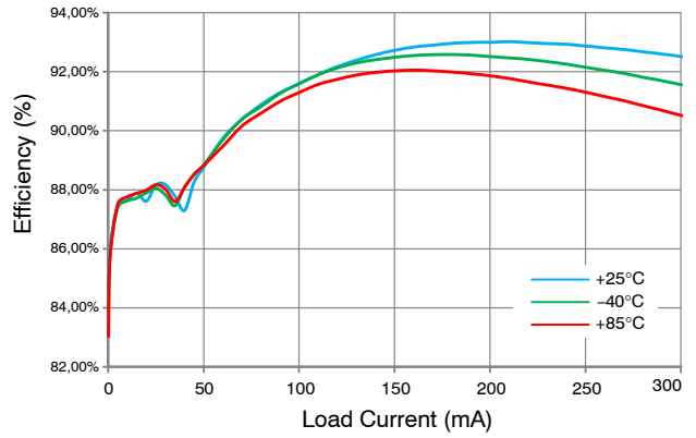
Figure 6. Efficiency vs. Temperature, 3.6 V IN
