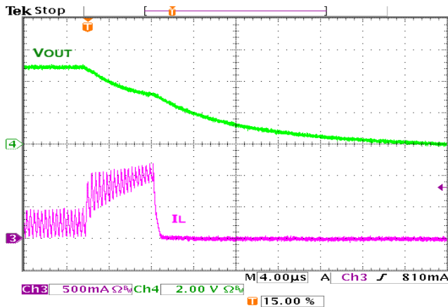
Figure 33. Overload Protection
