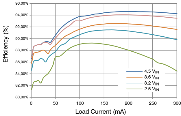
Figure 5. Efficiency vs. V IN
