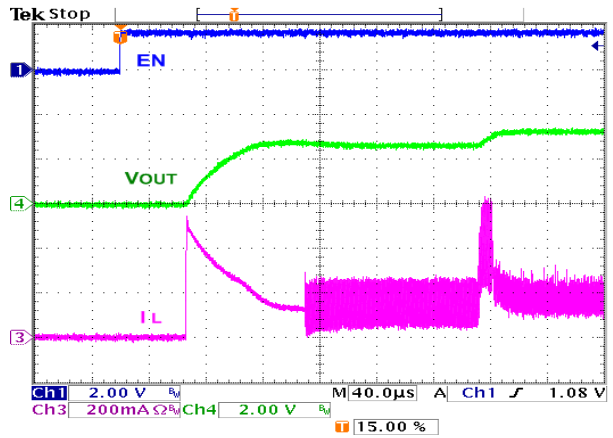
Figure 44. Startup, 22 Ω Load
