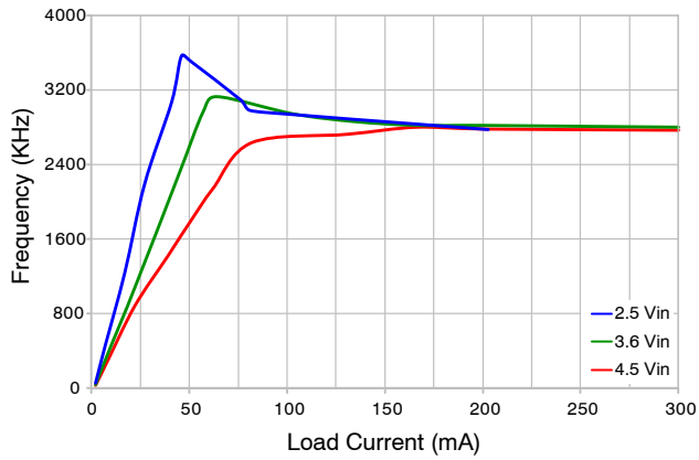
Figure 19. Switching Frequency
