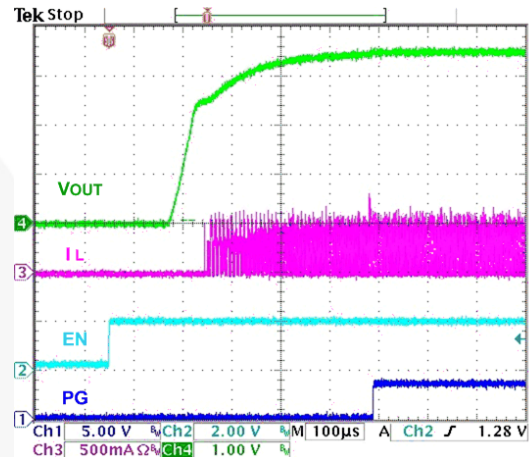
Figure 18. Startup, 50 Ω Load, V_{IN}=2.5\text{ V} , V_{OUT}=3.5\text{ V}
