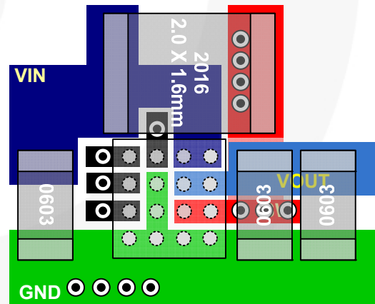
Figure 29. Layout Recommendation
