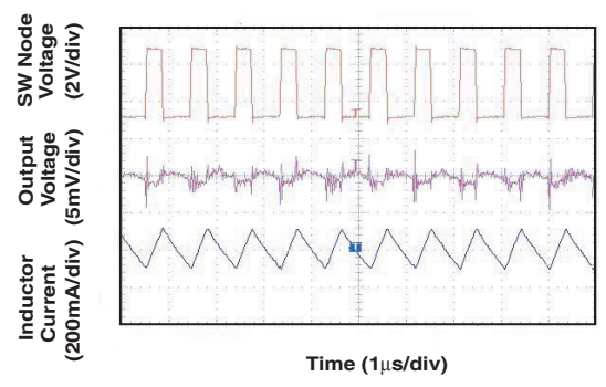
Figure 9. PWM Mode
