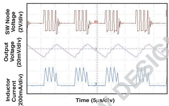
Figure 10. Power-Save Mode
