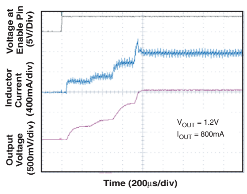
Figure 14. Start-Up Response
