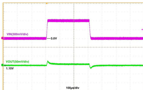
Figure 12. Line Transient, V_{IN} = 3.0\text{ V} \leftrightarrow 3.6\text{ V} , T_R = T_F = 10\text{ μs} , I_{OUT} = 500\text{ mA}
