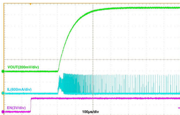
Figure 13. Startup, R_{load} = 50\text{ Ω}
