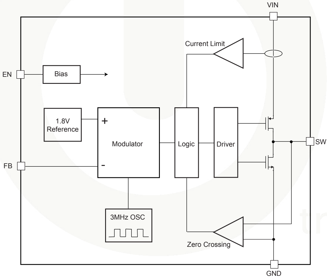
Figure 3. Block Diagram
