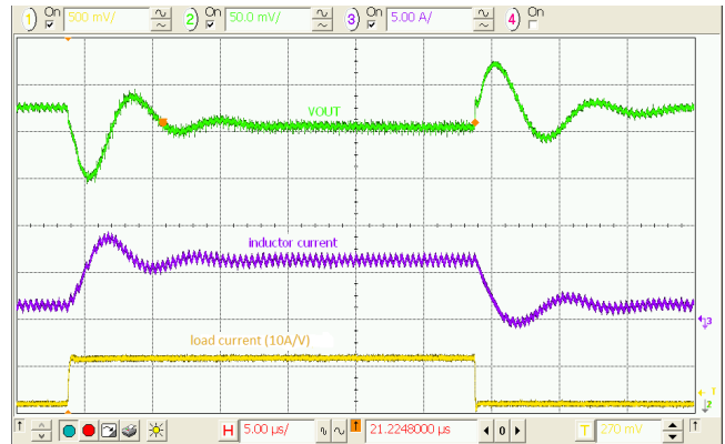
Figure 28. Load Transient, 3.6\text{ V}_{IN} , 1.2\text{ V}_{OUT} , 1.5\text{--}6\text{ A} , 100\text{ ns Edge} , C_{OUT} = 4 \times 22\ \mu\text{F}
