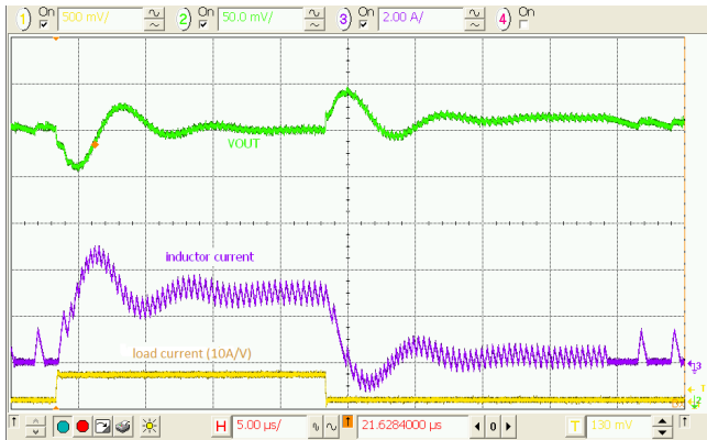
Figure 27. Load Transient, 3.6\text{ V}_{IN} , 1.2\text{ V}_{OUT} , 0.3\text{--}3\text{ A} , 100\text{ ns Edge} , C_{OUT} = 4 \times 22\ \mu\text{F}
