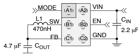
Figure 1. Typical Application
