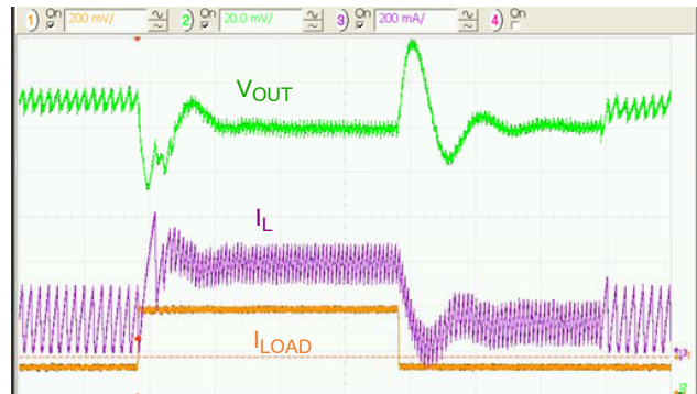
Figure 22. Load Transient 150 mA to 400 mA, V_{IN} = 3.6\text{ V} , t_{RISE} = t_{FALL} = 100\text{ ns} , 5 \mu\text{s} /div.
