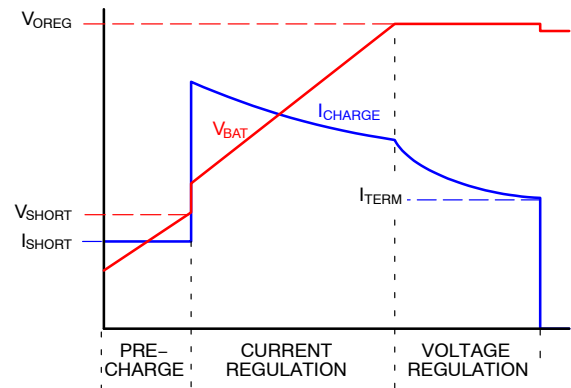
Figure 34. Charge Curve, I NLIM Limits I CHARGE
