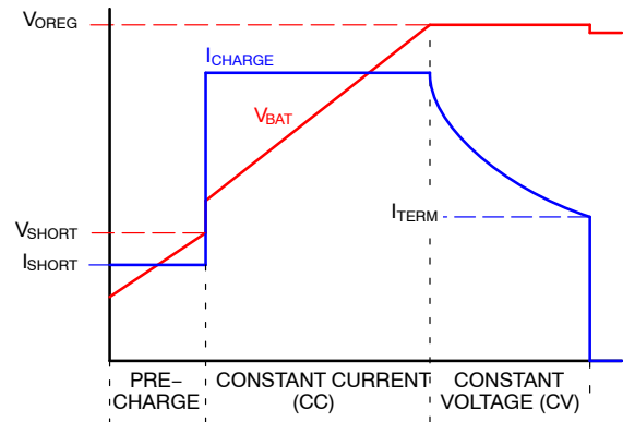
Figure 33. Charge Curve, I CHARGE Not Limited by I NLIM
