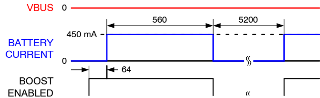
Figure 41. Boost Response Attempting to Start into VBUS Short Circuit (Times in μs)
