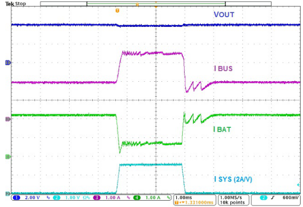
Figure 9. Load Transient Response, [\text{IBATREG}] = 2\text{ A} , [\text{IBUSREG}] = 3.5\text{ A} , T_A Configured for 5 V/5 A
