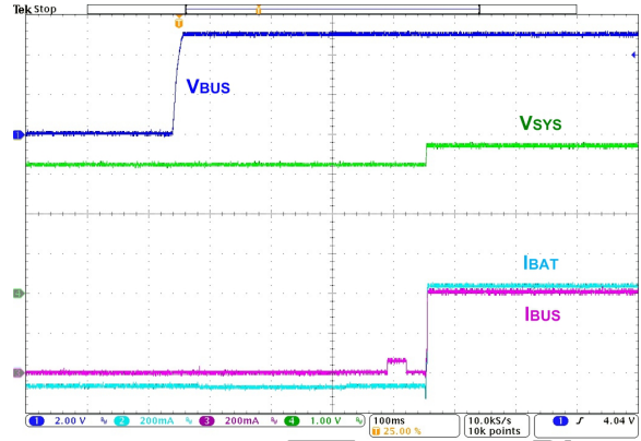
Figure 20. FAN545110 Startup at V_{BUS} Plug-In, V_{BAT} = 3.2\text{ V} , 50\ \Omega SYS Load, SDP, No Host Control
