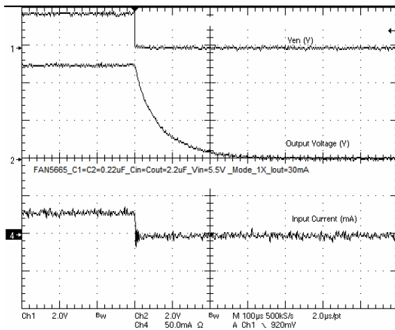
Figure 26. Turn-off at I_{OUT} = 30\text{mA} in 1x Mode
