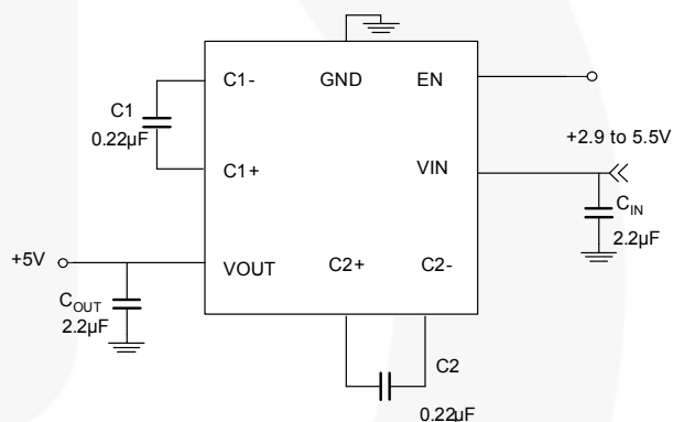
Figure 1. Typical Application
