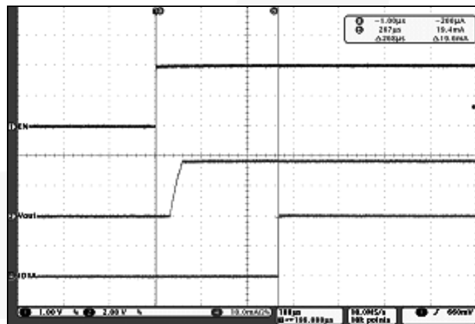
Figure 15. Soft-Start with EN, V_{IN}=3.6V , I_{LEDx}=20mA
