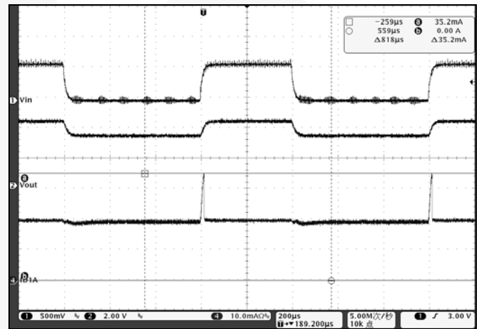
Figure 13. Line Transient Response in 1.5x Mode, V_{IN}=2.7V - 3.3V , I_{LEDx}=20mA
