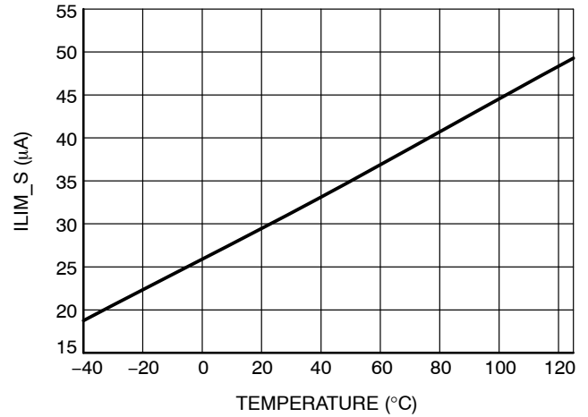
Figure 19. 30 μA Current Source for Current Limit Purpose vs. T at V_{\text{HVBIAS}} = 48\text{ V}
