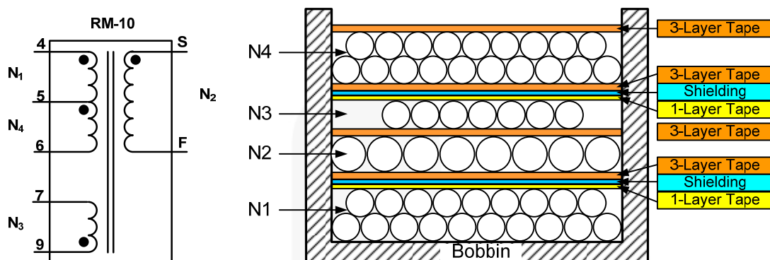
Figure 41. Transformer Specification
