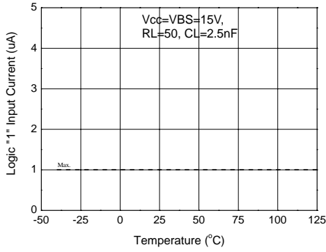
Figure 16a. Logic "1" IN Current vs Temperature
