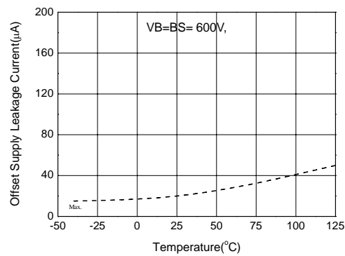
Figure 12a. Offset Supply Leakage Current vs Temperature
