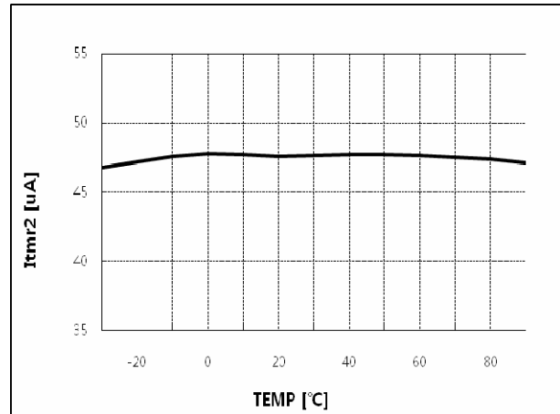
Figure 34. TIMER Current 2 vs. Temperature
