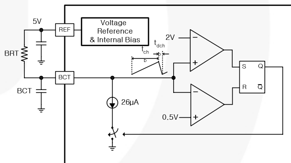
Figure 36. Burst Dimming Oscillator Circuit
