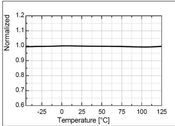
Figure 19. OVP Threshold at OVP Pin ( V_{OVP,OV} ) vs. T_A
