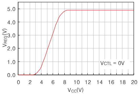
1. V_{CC} vs V_{REG}
