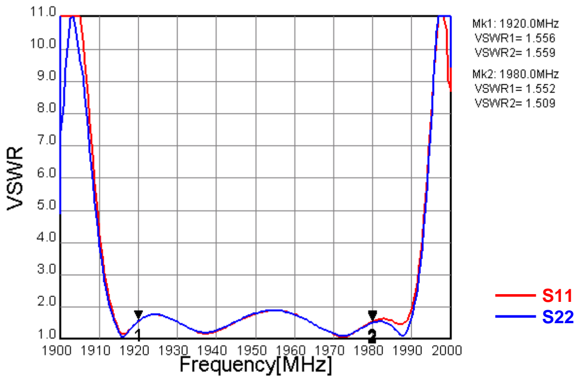
Fig.2 VSWR
