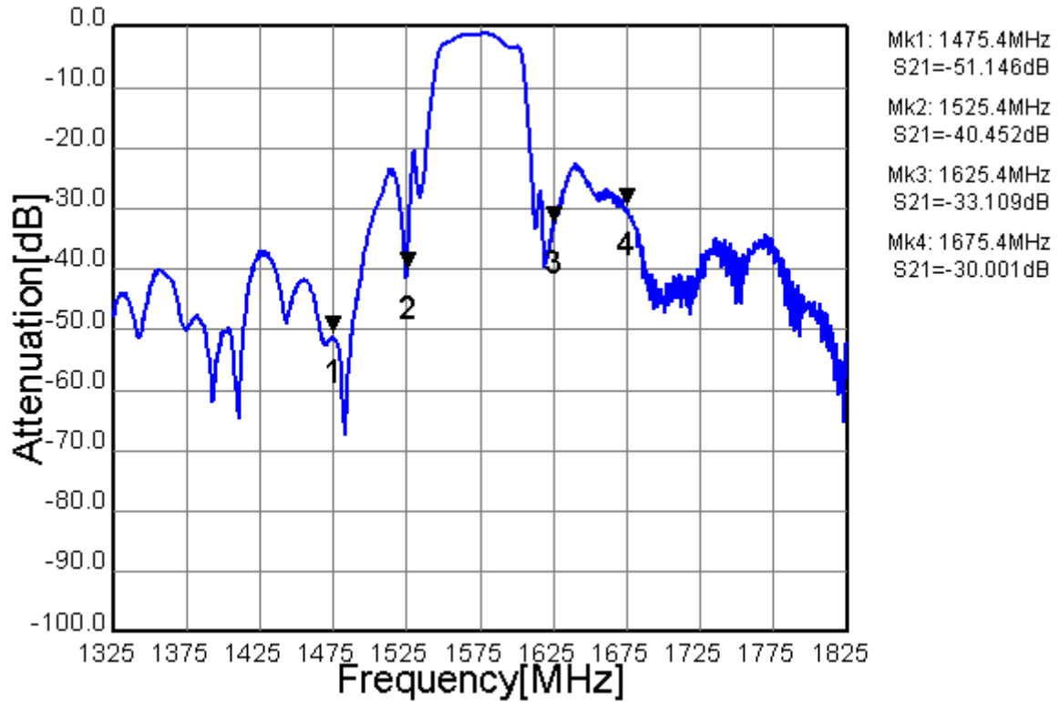
Fig.1 Pass-band Characteristic
