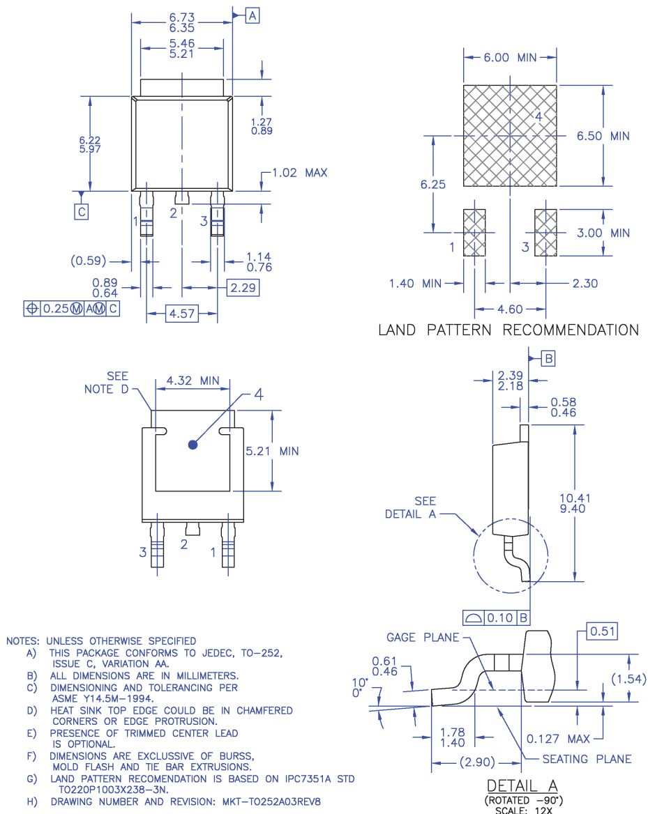
Figure 17. TO252 (D-PAK), Molded, 3-Lead, Option AA&amp;AB
