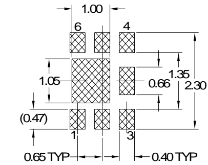
RECOMMENDED LAND PATTERN OPT 2
