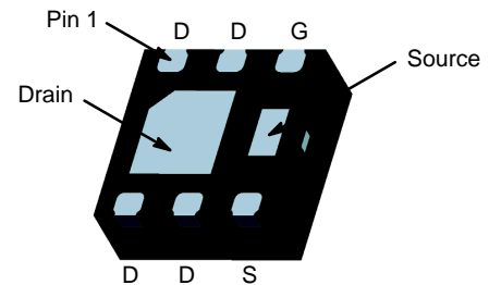
WDFN6 2x2, 0.65P (MicroFET 2x2) CASE 511CZ
