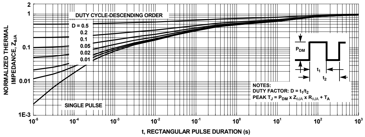
Figure 24. Transient Thermal Response Curve
