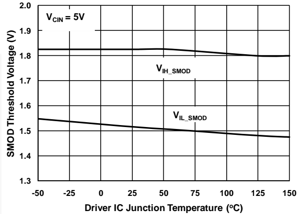
Figure 19. SMOD# Thresholds vs. Temperature
