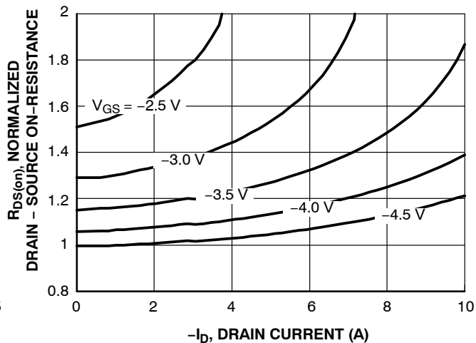
Figure 2. On-Resistance Variation with Drain Current and Gate
