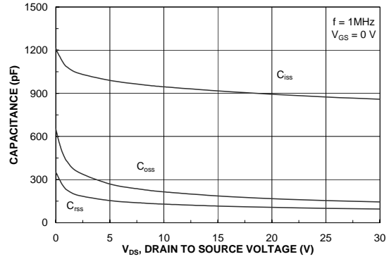
Figure 22. Capacitance Characteristics.
