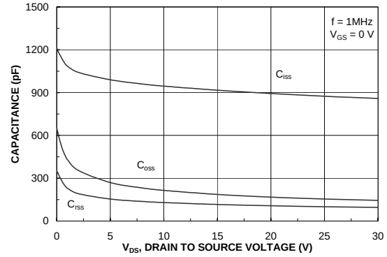
Figure 22. Capacitance Characteristics.
