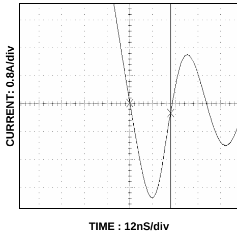
Figure 12. FDQ7238AS SyncFET body diode reverse recovery characteristic.
