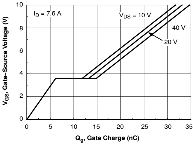
Figure 7. Gate-Charge Characteristics
