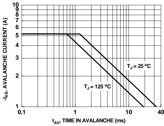
Figure 23. Unclamped Inductive Switching Capability
