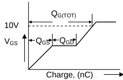
Figure 28. Gate Charge Waveform
