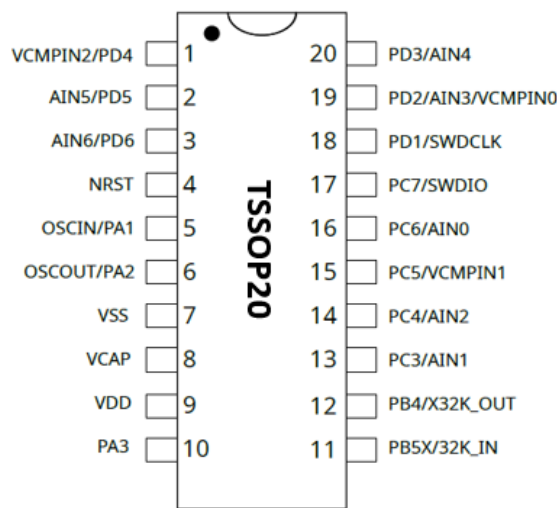
Figure 1. TSSOP20
