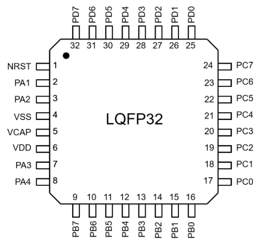
Figure 2. LQFP32
