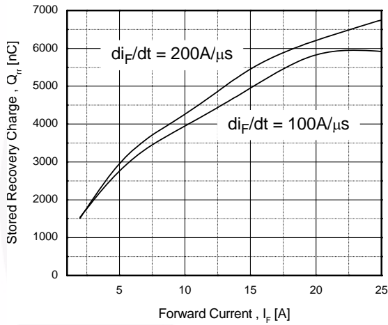
Figure 19. Stored Charge
