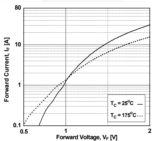
Figure 18. Forward Characteristics
