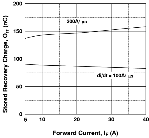
Figure 21. Stored Charge
