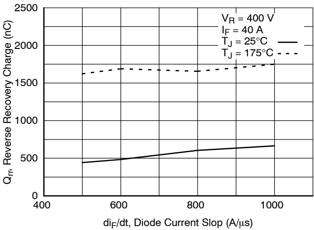
Figure 18. Stored Charge
