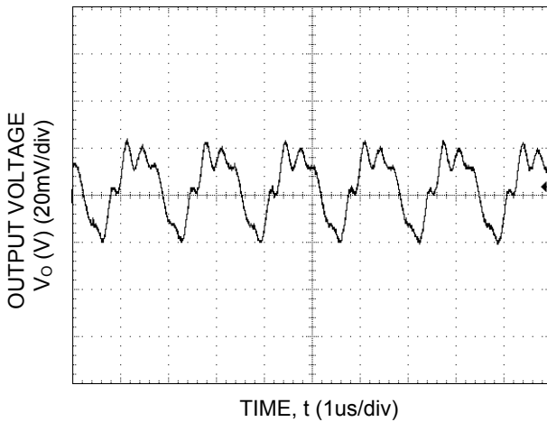
Fig-23. Typical output ripple and noise ( C_O=22\mu F ceramic, V_{IN} = 12V , I_o = I_{o,max} ).
