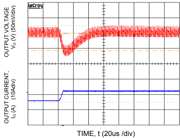
Fig-24. Transient Response to Dynamic Load Change from 50% to 100% at 12Vin, C_{out}= 1x47\mu F+1x330\mu F , C_{Tune}=2700pF & R_{Tune}=330ohms
