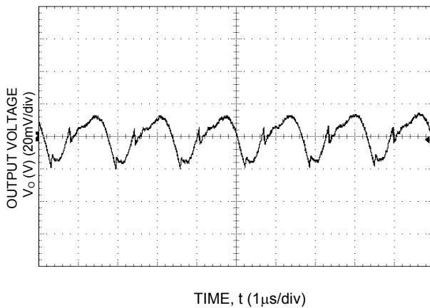
Figure 27. Typical output ripple and noise ( C_o=10\mu F ceramic, V_{IN} = 12V , I_o = I_{o,max} , ).
