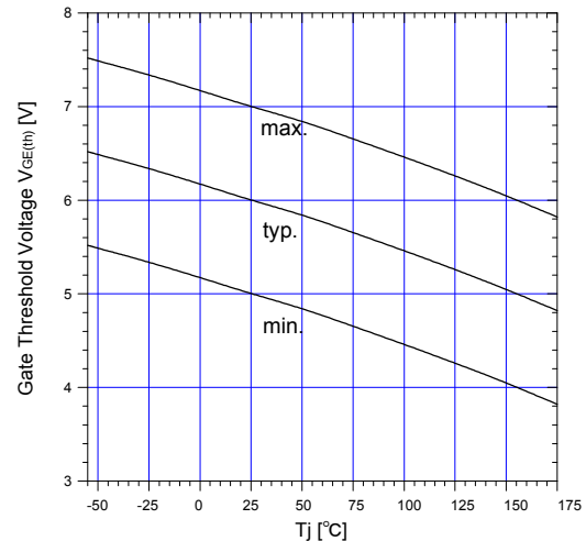
Graph.6 Gate Threshold Voltage vs. T_j I_C = 40mA, V_{CE} = 20V
