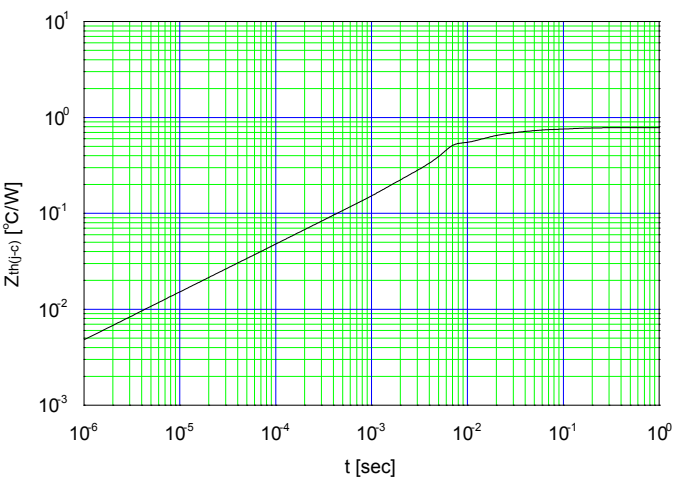
Graph.18 Transient thermal resistance of FWD
