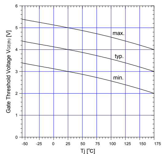
Graph.6 Gate Threshold Voltage vs. T_j I_C=75mA , V_{CE}=20V
