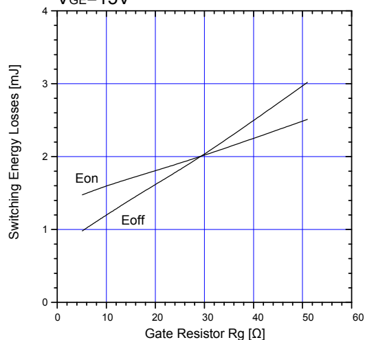
Graph.12 Typical switching losses vs. R_g T_j=150^\circ C , V_{cc}=400V , I_c=37.5A , L=500\mu H V_{GE}=15V
